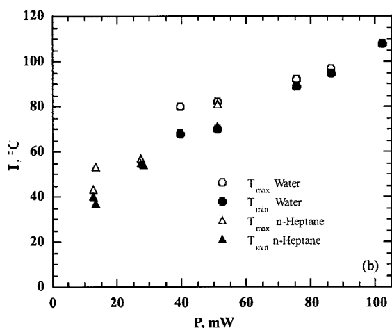
Figure 4. (a) Bubble growth data and the associated temperature decay of the heating thermistor during a heat pulse; (b) maximum and minimum thermistor temperatures during heat pulses vs. the power delivered.
