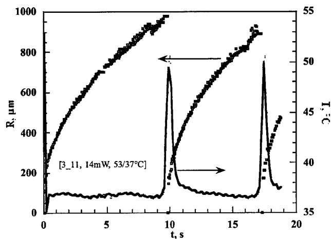
Figure 6. Three bubbles growing one after the other in n -heptane.
